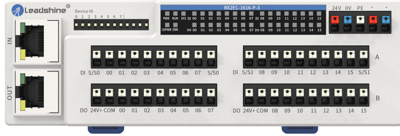
RX2EC-1616-P-3
